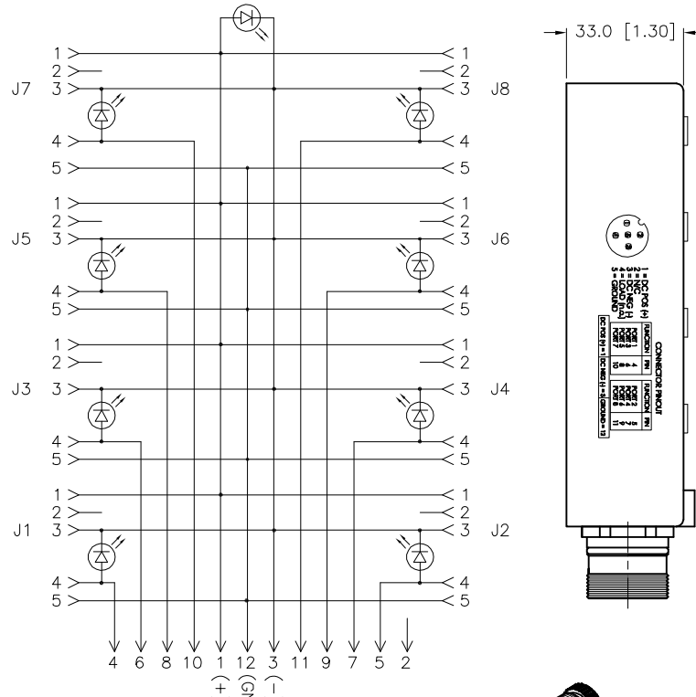
WIRING DIAGRAM
